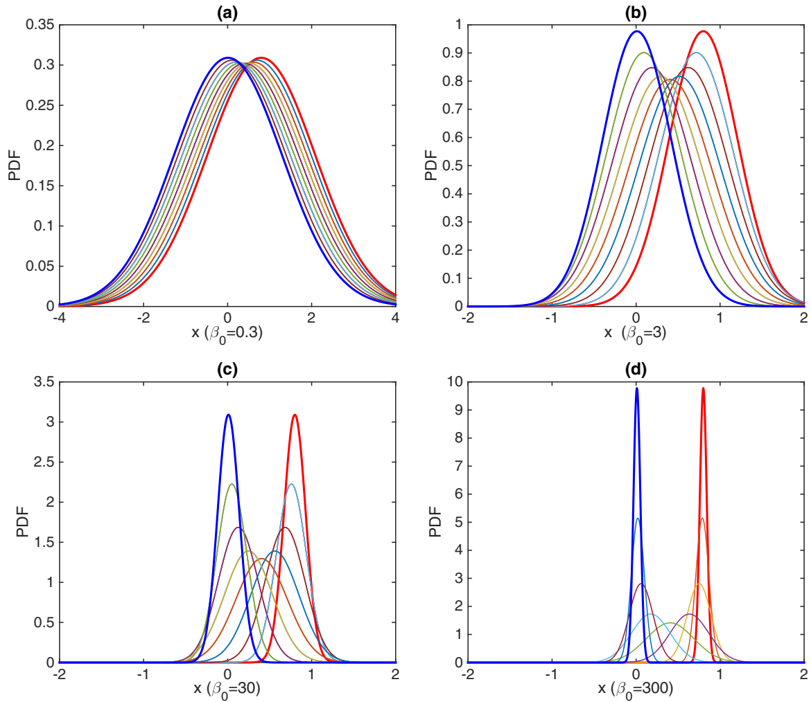
FIG. 4. Time evolution of PDFs against x for \beta_0 = 0.3, 3, 30, \text{ and } 300 in (a)–(d), respectively. y_0 = \langle x(t=0) \rangle = 5/6 and y_F = \langle x(t=t_F) \rangle = 1/30 . The initial and final PDFs are shown by thick red lines on the right and blue lines on the left, respectively.
