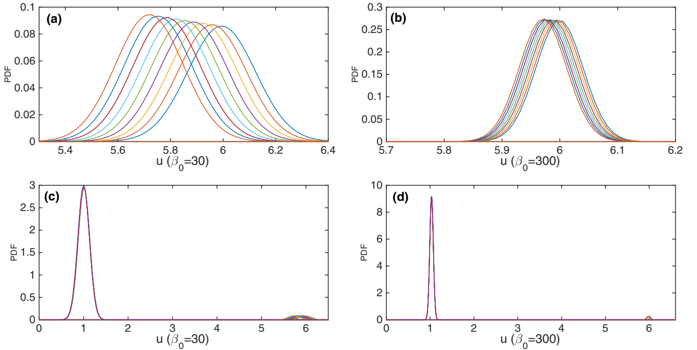
FIG. 8. Time evolution of PDFs of the population u for \beta_0 = 30 and 300 , corresponding to Fig. 7. \langle u(t=0) \rangle = 6xs\langle u(t=t_F) \rangle = 1.0345 , which is close to the carrying capacity u_\infty = 1 ( \gamma = 1 , \epsilon = 1 ). (a)–(b) show the PDF during the first cycle as in Figs. 7(a)–7(b), where the PDF at t = 0 can be identified with the peak at u = 6 . (c)–(d) are the evolution of PDFs over the first and the last cycles [tenth and hundredth cycle for (c) and (d), respectively] shown at the same time.
