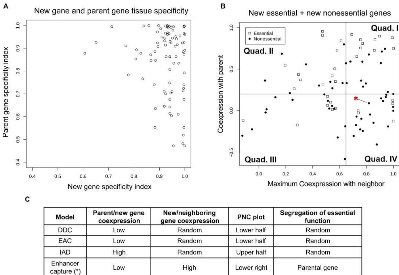
Fig. 2. Asymmetrically duplicated new genes evolve via enhancer capture. (A) Using new-gene/parent-gene pairs for genes evolving via distal duplication in D. melanogaster , the tissue specificity index \tau is calculated and plotted above, demonstrating that new genes evolving via distal duplication have higher tissue specificity than parental genes. (B) Shown are PNC patterns for new genes in D. melanogaster , which have duplicated either more than 500 kb away or between chromosomes. Tissue coexpression (Spearman correlation coefficient) between new gene/parental gene pairs is plotted on the vertical axis, while maximal tissue coexpression between new gene/neighboring genes pairs is plotted on the horizontal axis. Vertical and horizontal lines indicate median coexpression value of all distally duplicated new genes presented here. Genes that evolved via enhancer capture are expected to have low parental coexpression and high neighboring coexpression and should thus be present in the lower-right quadrant. (C) While a new gene's essential function is equally likely to be partitioned between either parent or new gene under prior models, new genes evolving via enhancer capture are unlikely to have essential functions, as the expression of the new gene will only augment existing expression of the parental gene, leaving the original essential function intact. Comparing the ratio of new essential to new nonessential genes (29:36, 44.6%) in quadrants I to III to the ratio of new essential to new nonessential genes in quadrant IV showing high neighboring/low parental coexpression (5:17, 22.7%) shows that new genes likely evolve via regulatory capture (2.18-fold enrichment, P = 0.0055 , 2D K-S test). (*) denotes HP6/Umbrea .
